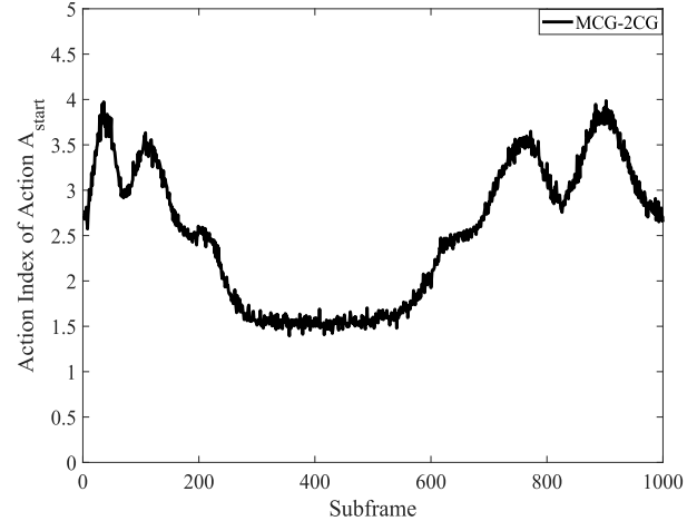
Fig. 15. Action index of the action A_{start} in the action set \mathcal{A}_{start} for MCG-GF-NOMA with N_{CG} = 2 .
