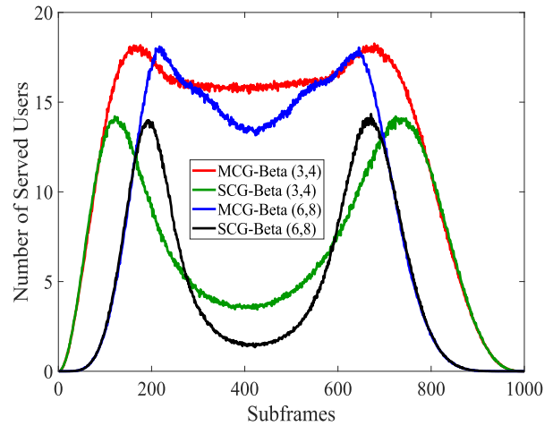
Fig. 7. Average number of successfully served users in high traffic scenario.
