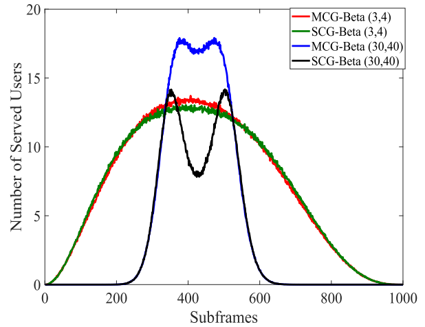
Fig. 6. Average number of successfully served users in low traffic scenario.
