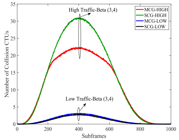
Fig. 10. Average number of collision CTUs.
